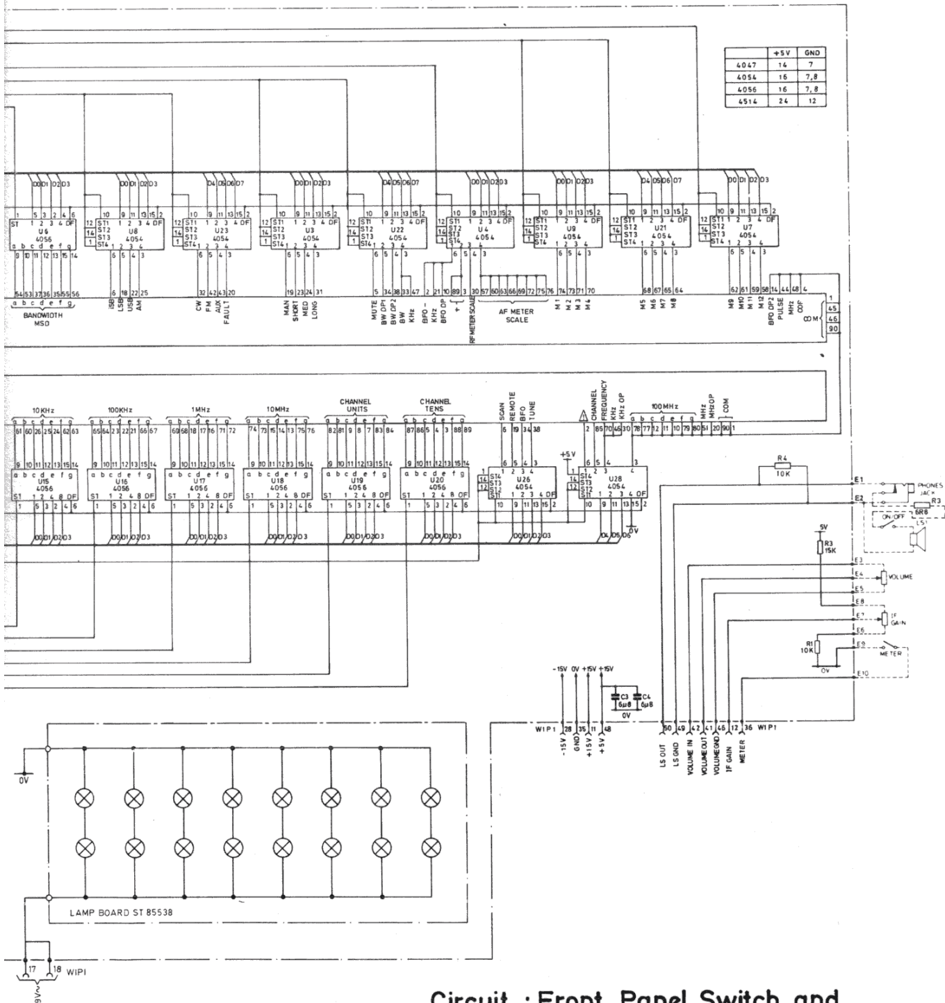
Circuit : Front Panel Switch and Display Board A9A1 Fig.9.1
